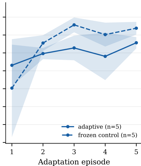
AttentivePPO-clip
