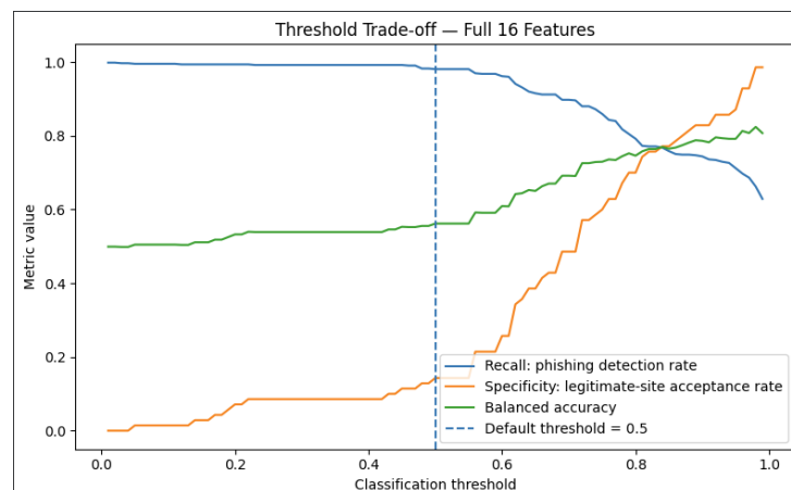
Figure: Trade-off between phishing recall, legitimate-site specificity, and balanced accuracy across XGBoost classification thresholds using the full 16-feature representation.
