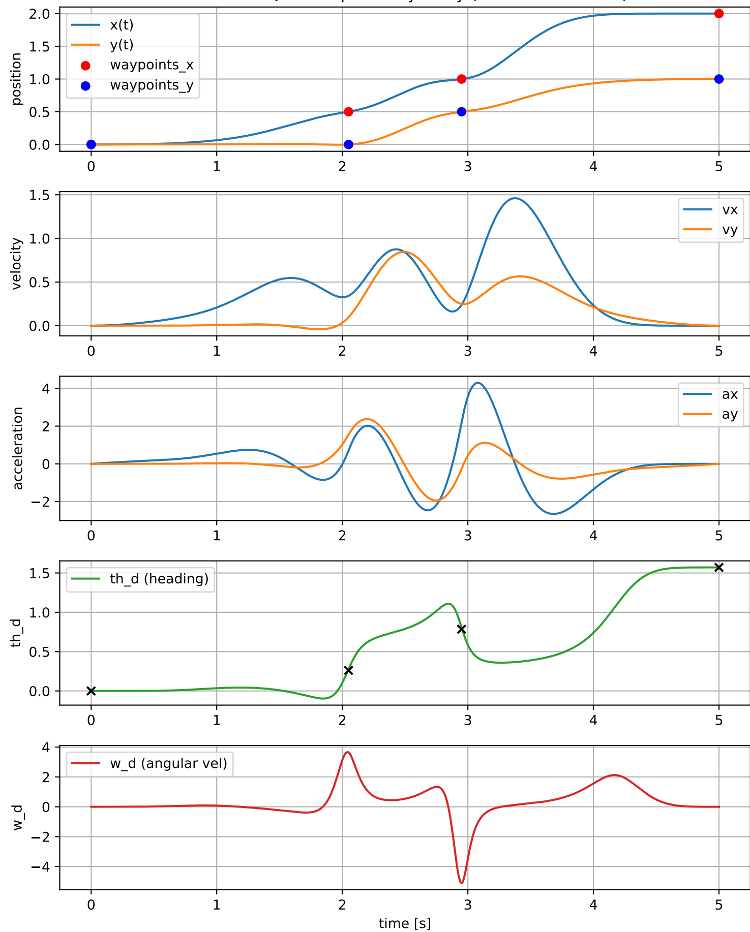
Path-Time Quintic Spline Trajectory ( \theta at selected WPs)
