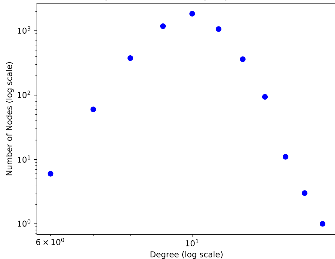
Degree Distribution (Log-Log) - net1.net
