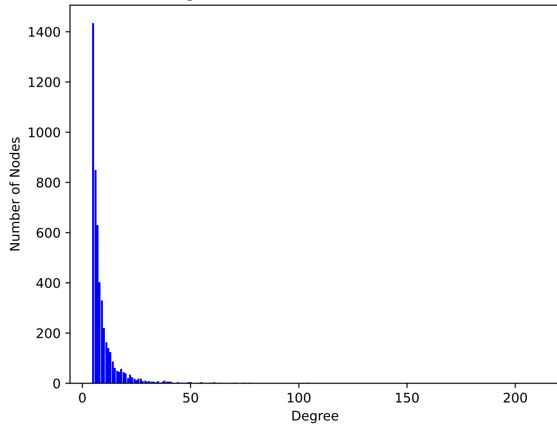
Degree Distribution (Linear) - net4.net
