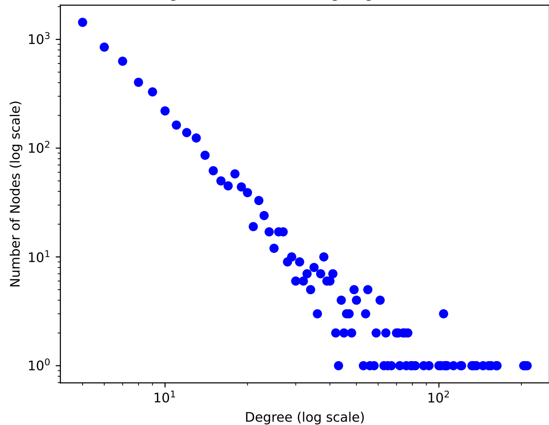
Degree Distribution (Log-Log) - net4.net
