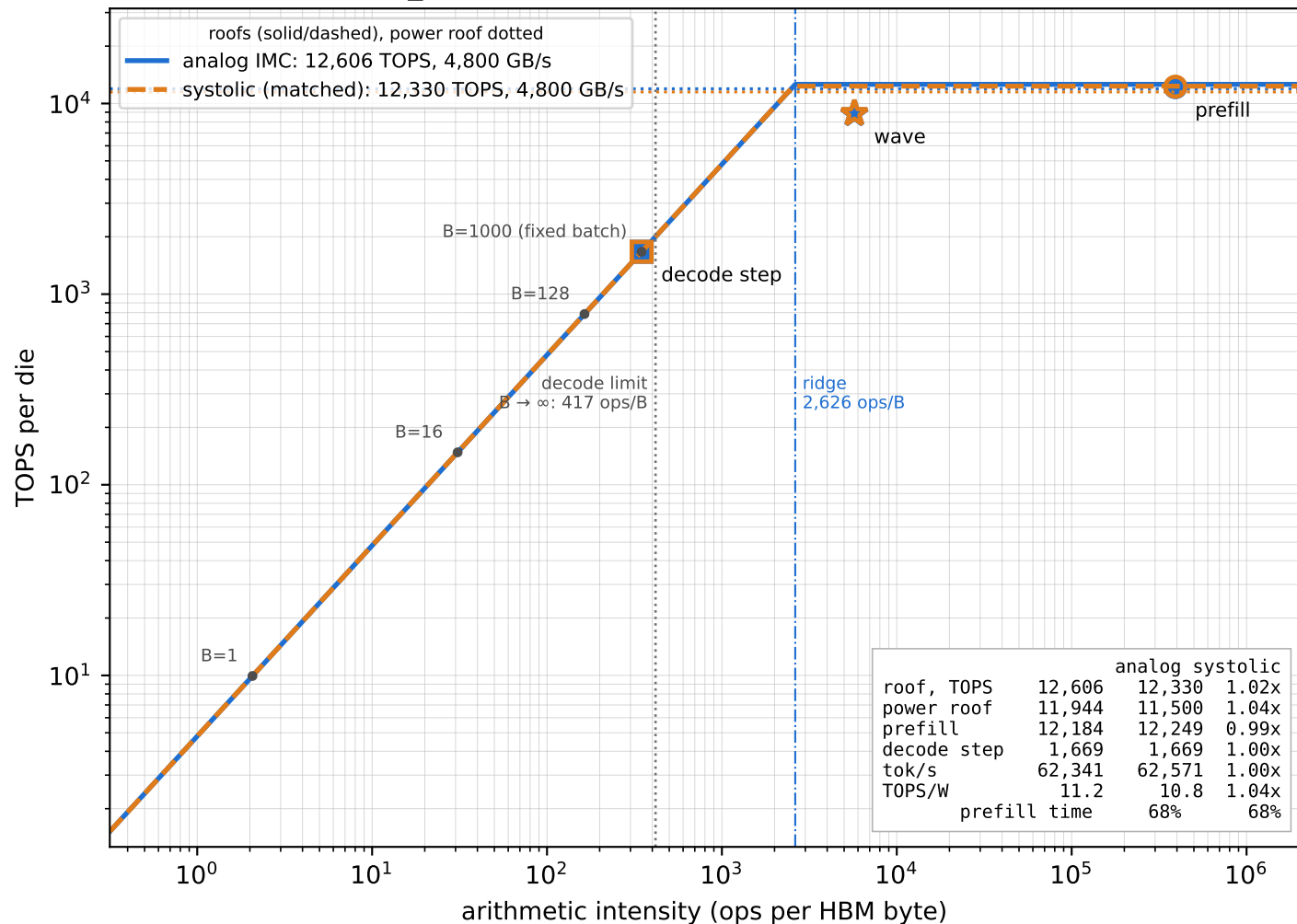
Sohu: Llama-3-70B FP8, 2048/128, B=1000, 1,063 mm 2 , 4.8 TB/s (per die of 8) analog notes_native vs systolic W8 (same weight and KV formats)
