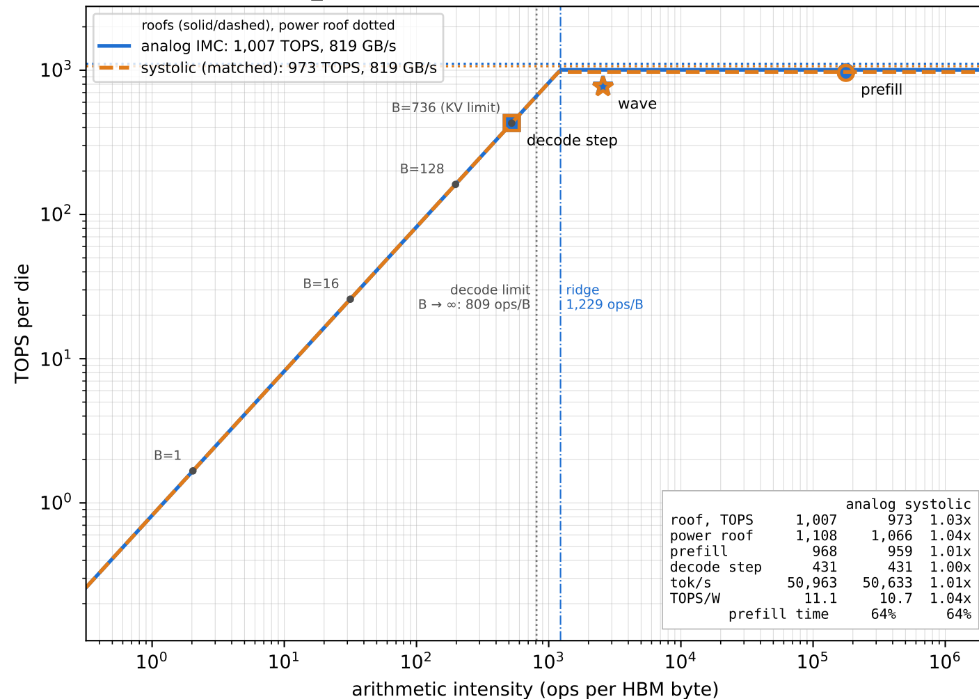
ARCH: Llama-3-8B, 512/128, 100 mm 2 , 1 HBM3 stack analog notes_native vs systolic W8 (same weight and KV formats)
