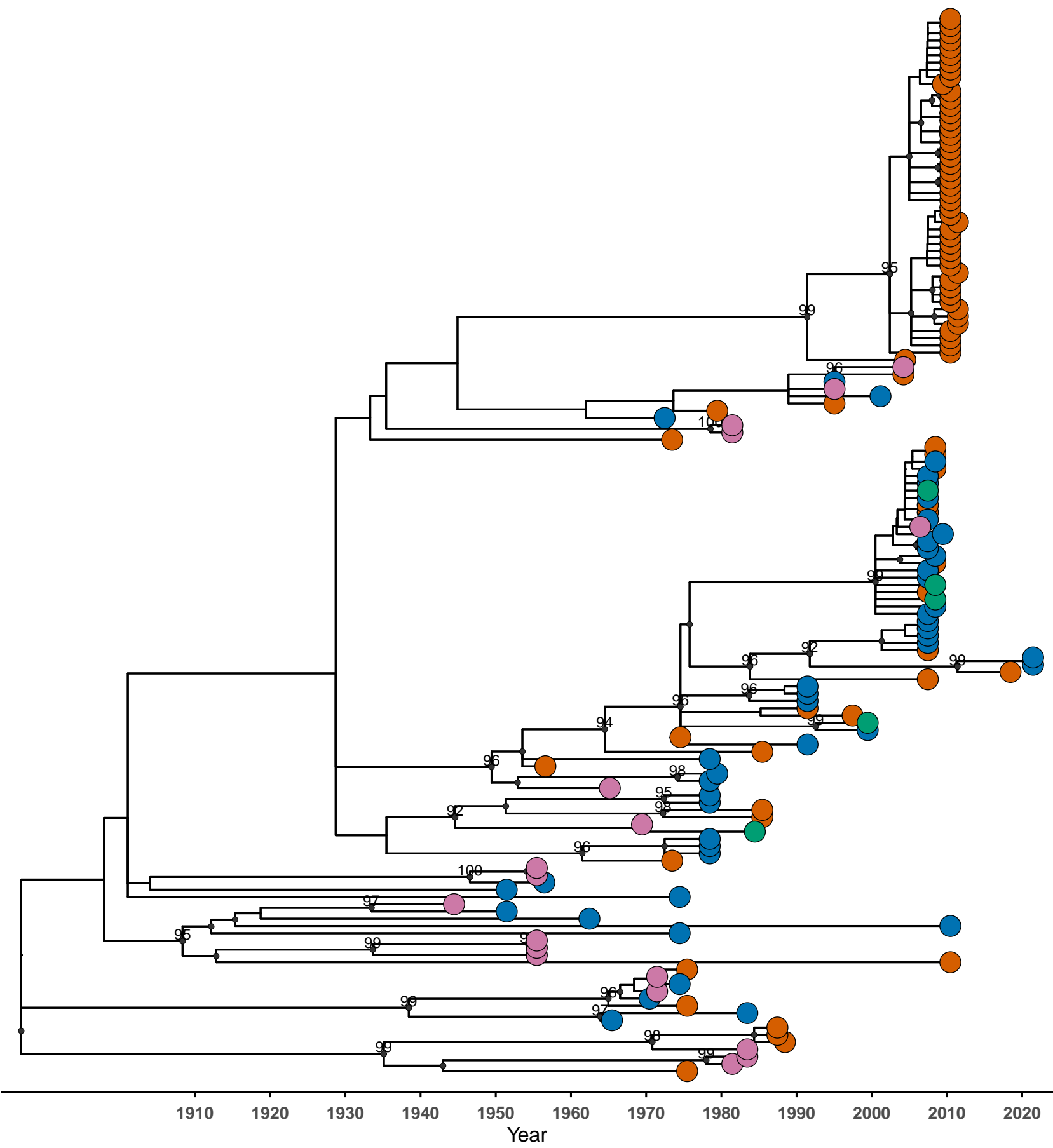
Host–Associated Phylogenetic Structure of RVFV S Segment
