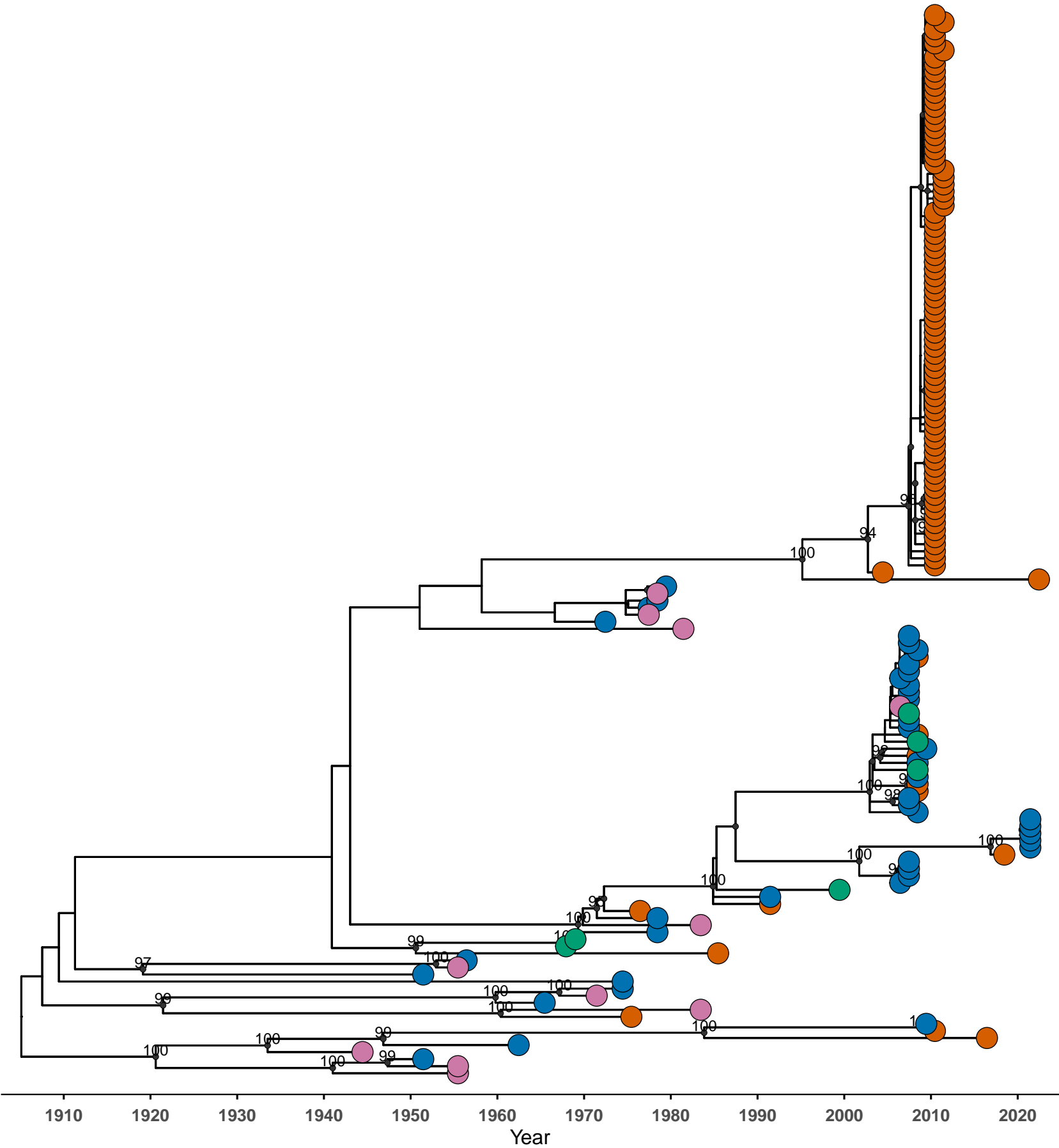
Host-Associated Phylogenetic Structure of RVFV L Segment
