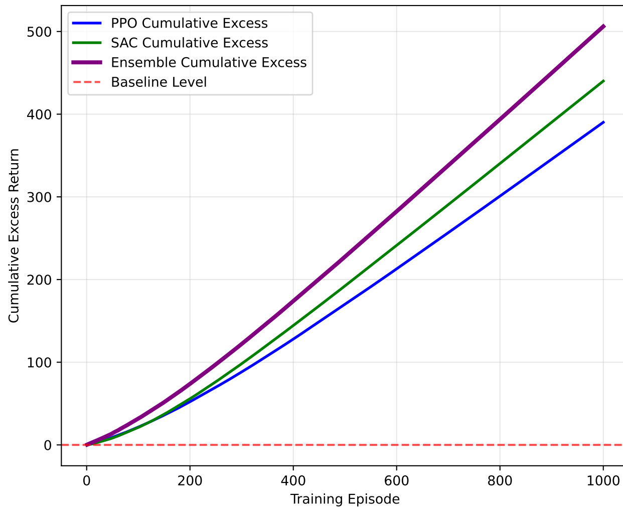
Cumulative Excess Performance
