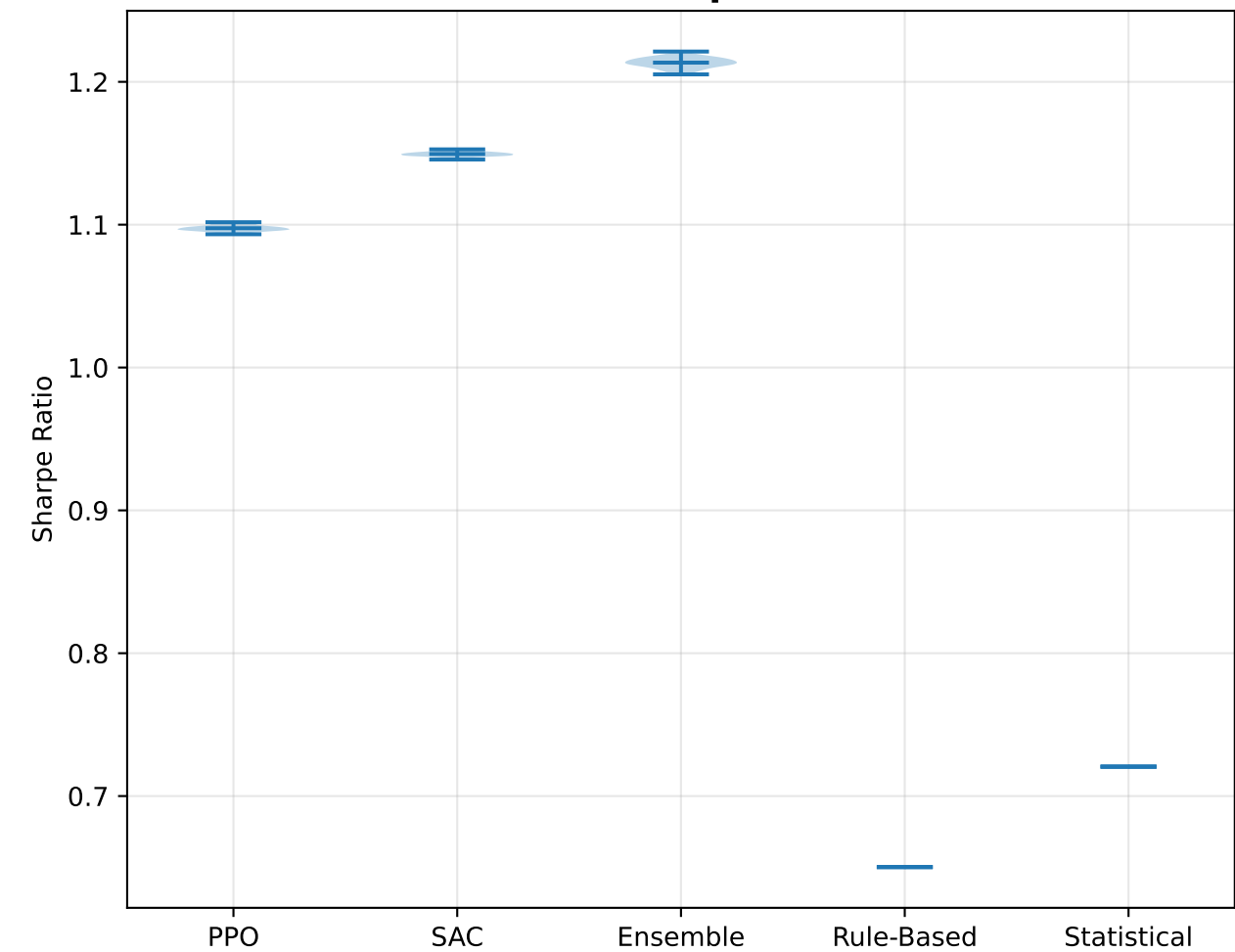
Final Performance Distribution (Last 100 Episodes)
