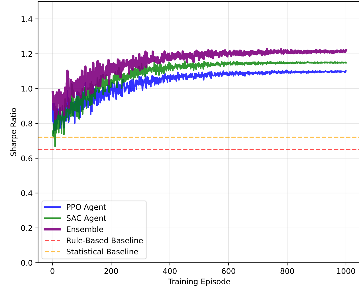
Sharpe Ratio Convergence
