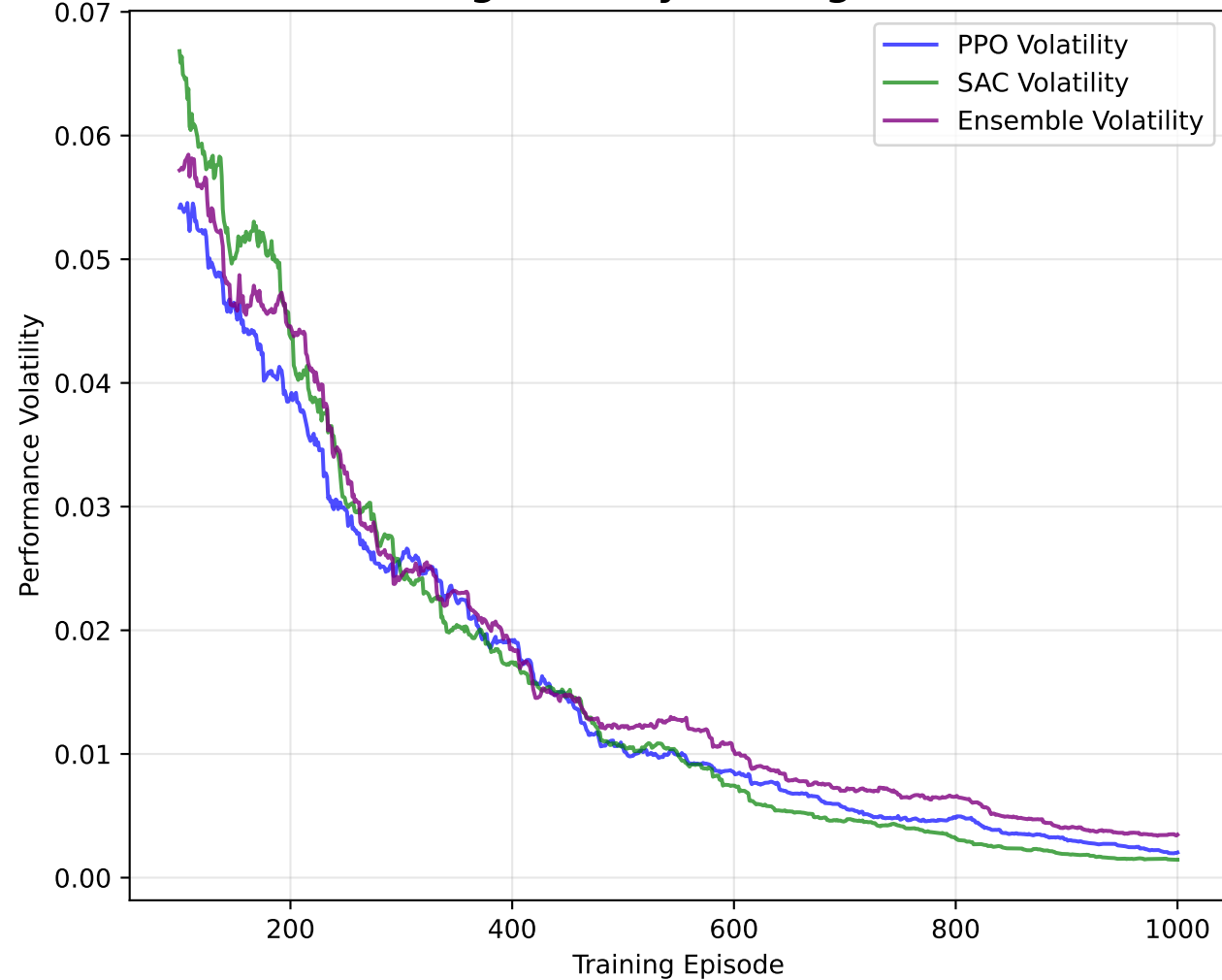
Learning Stability (Rolling Std Dev)
