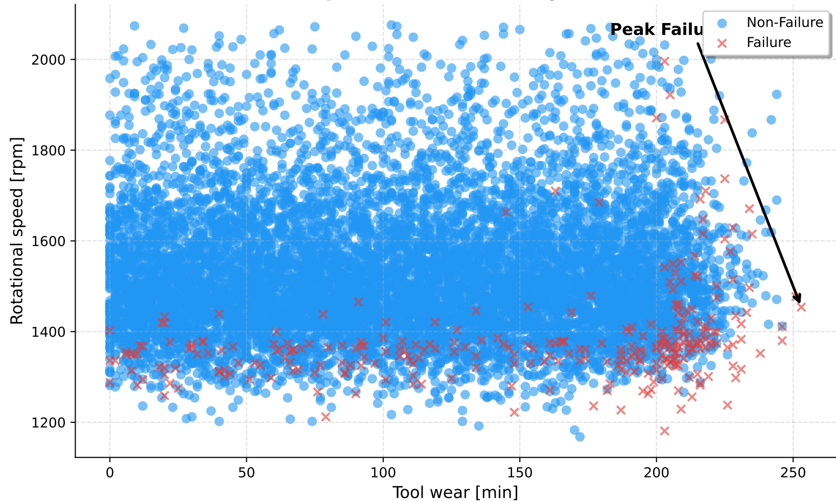
Rotational Speed vs. Tool Wear by Failure Status
