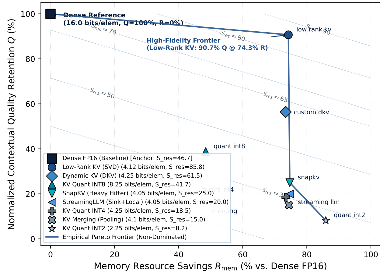
Context Quality Retention vs. Memory Resource Savings (0.5B Preliminary Profile)
