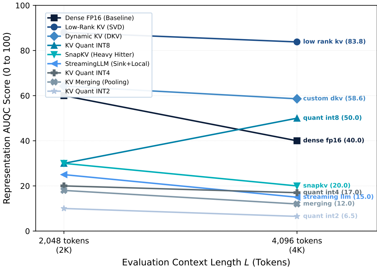
Context Representation Scaling from 2K to 4K Tokens (Measured 0.5B Profile)
