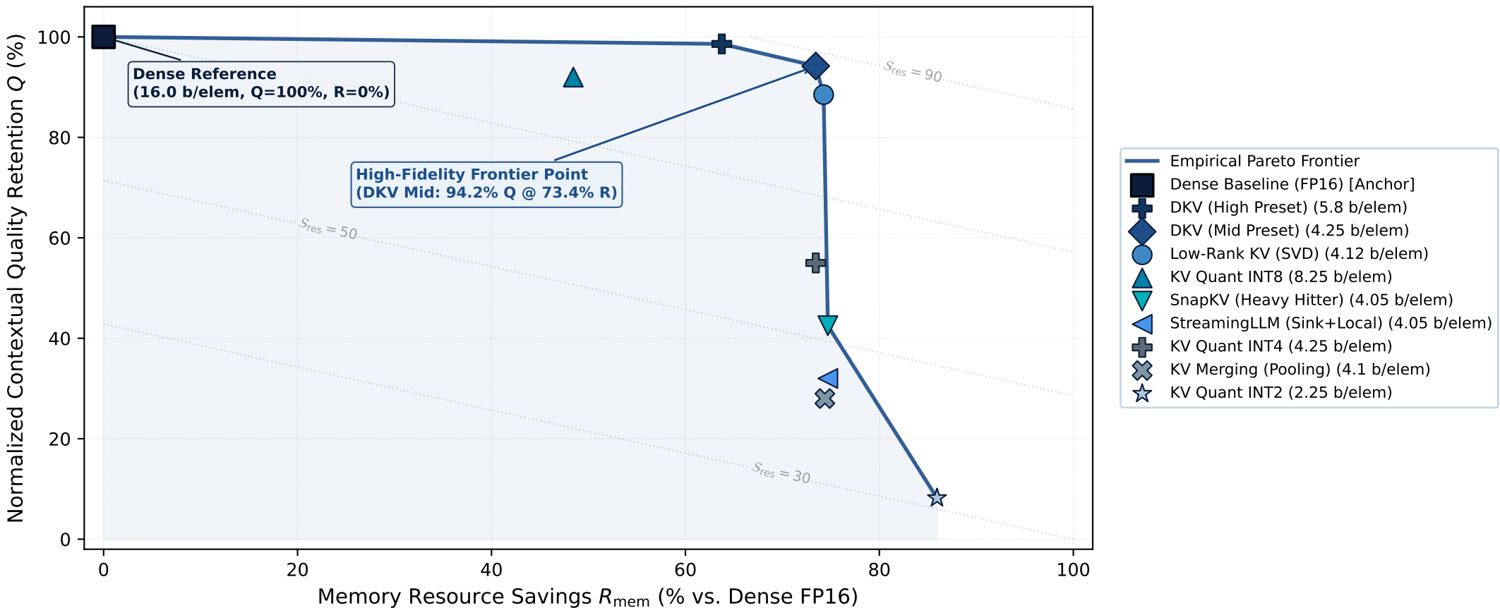
Context Quality Retention vs. Memory Resource Savings (1.5B Profile)
