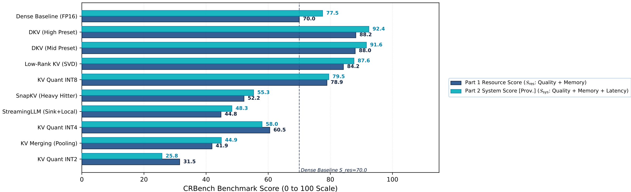
Preliminary Part 1 (Resource) vs. Provisional Part 2 (System) Scores on Qwen2.5-1.5B
