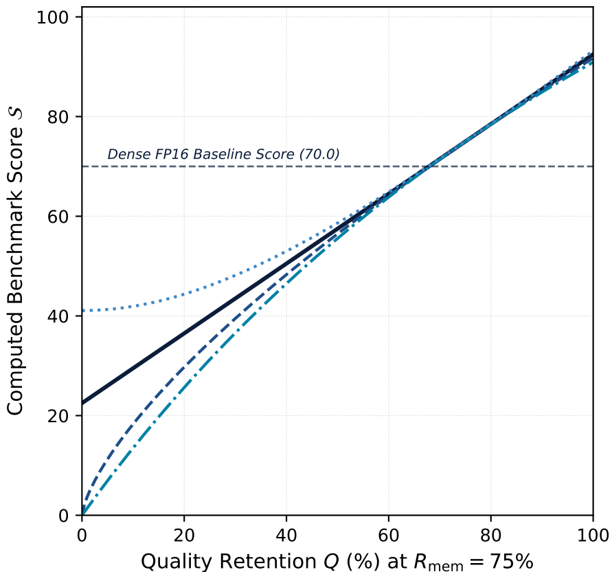
(a) Utility Formulations at Fixed R_{\text{mem}} = 75\%
