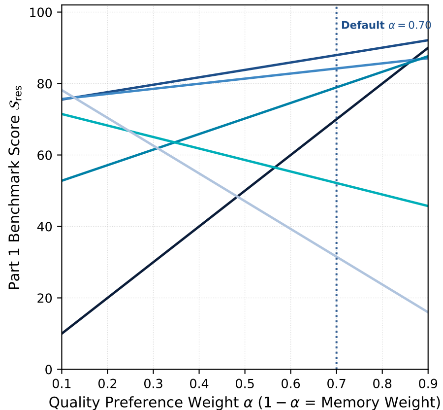
(b) Method Score Sensitivity across \alpha \in [0.10, 0.90]
