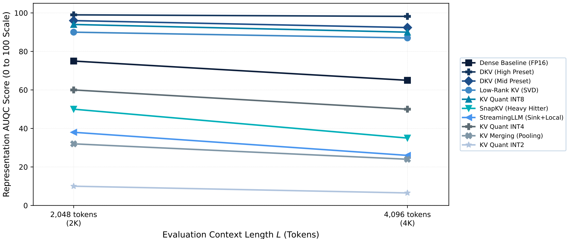
Context Representation Scaling from 2K to 4K Tokens (Measured 1.5B Profile)
