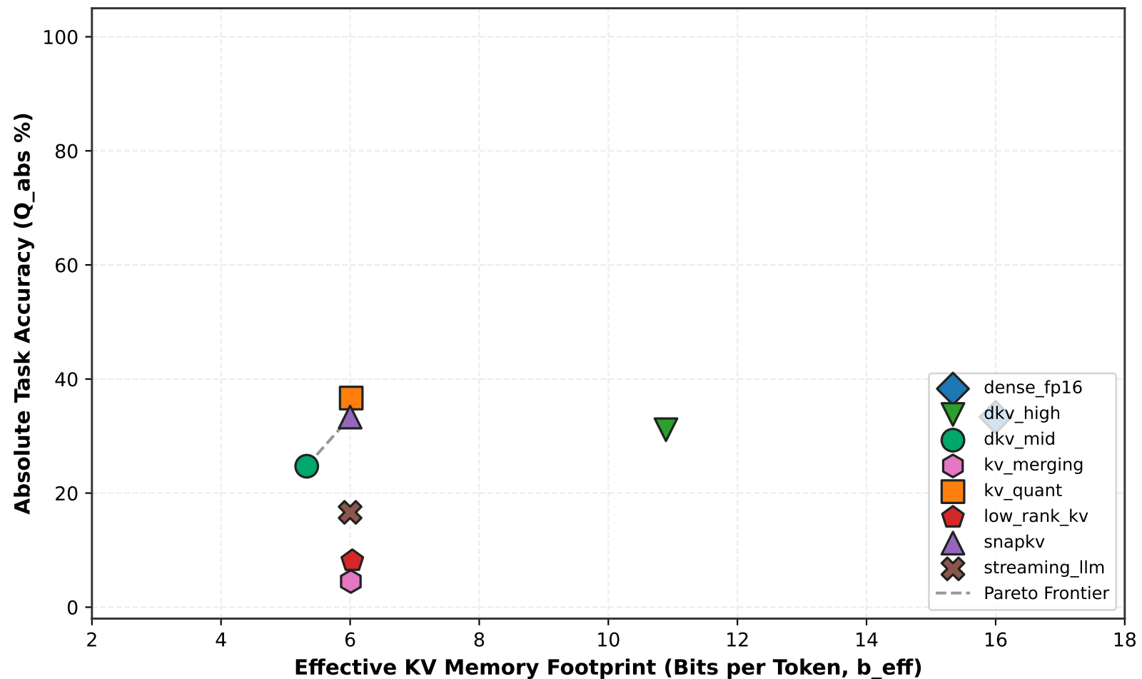
Qwen2.5 7B: Quality-Resource Tradeoff (32K Tokens)
