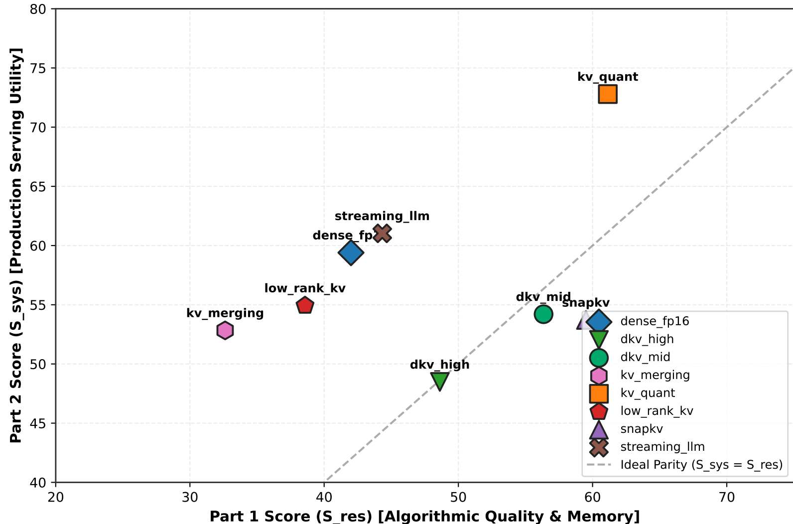
Qwen2.5 7B: Part 1 (S_res) vs. Part 2 (S_sys) Serving Utility
