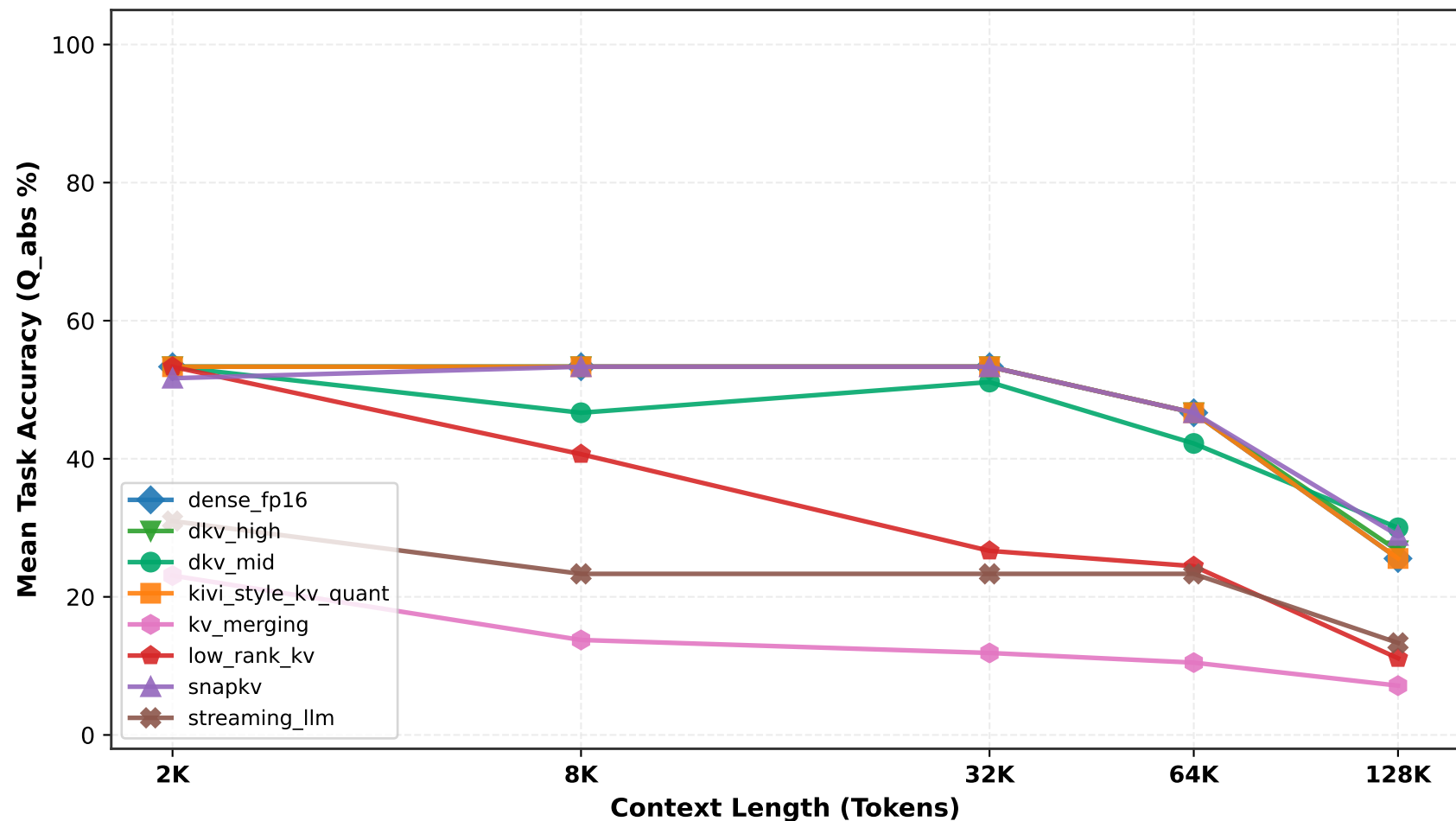
Gemma 4 E2B: Context Scaling Accuracy vs. Context Length
