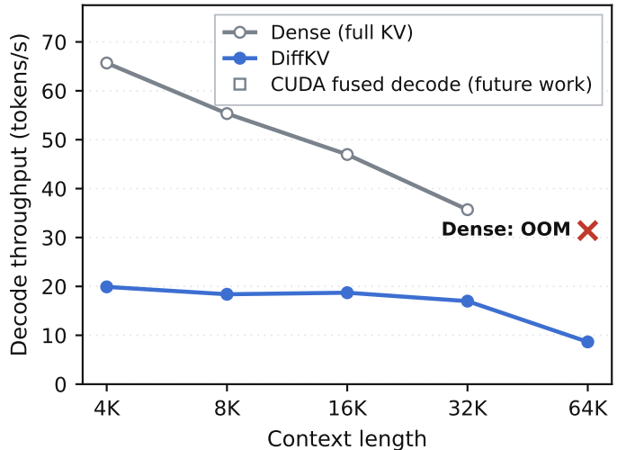
(b) Decoding
