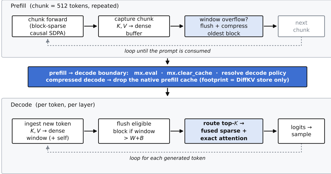
Figure 4 | Cache lifecycle. Prefill loops over chunks (attend, capture, flush-and-compress the oldest block on overflow). At the prefill \rightarrow decode boundary the runtime evaluates pending work, releases peak activations, and—on the compressed path—drops the native prefill cache. Decode then loops per token: ingest the new token into the window, flush an eligible block, and run the fused routed attention.
