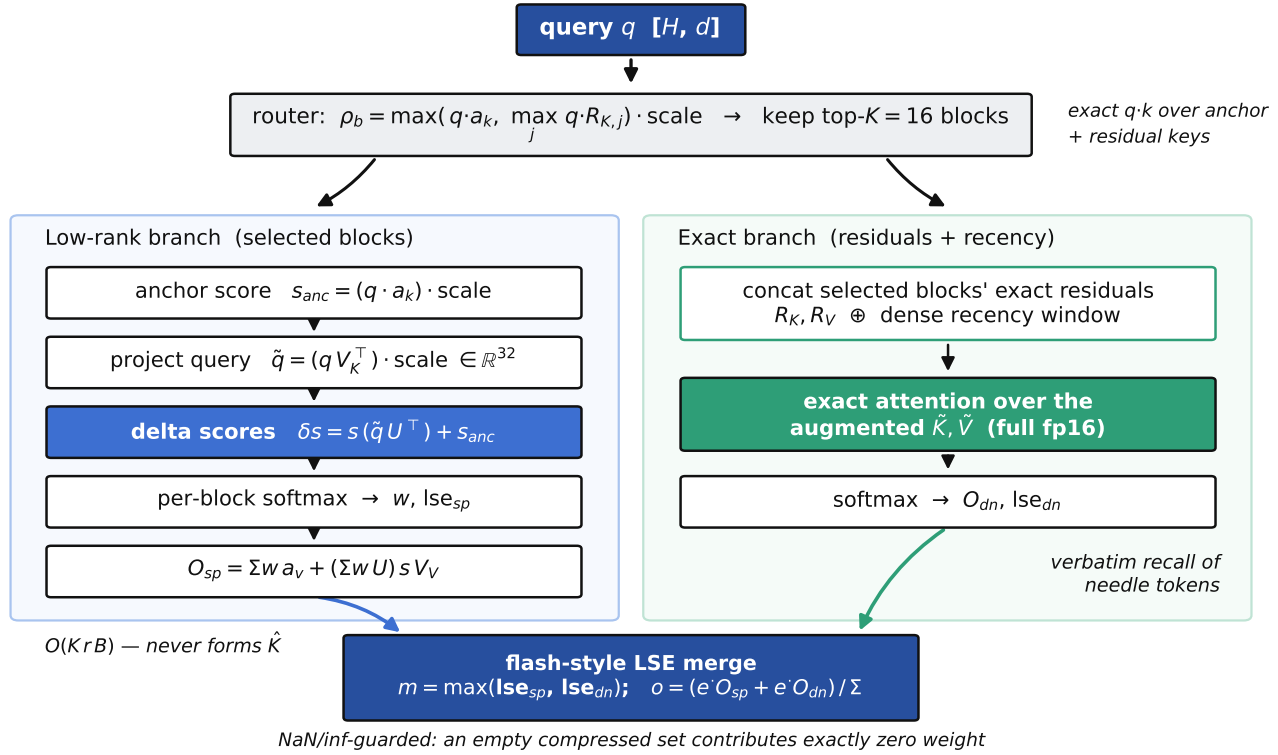
Figure 5 | The routed sparse decode kernel. A cheap exact router keeps the top- K blocks. Their contribution is computed in the rank- r subspace—anchor score plus a projected-query dot with U —without ever forming \hat{K} . In parallel, the selected blocks’ exact residuals and the dense recency window are attended directly. The two halves are combined by a flash-style log-sum-exp merge, guarded so an empty compressed set contributes exactly zero weight.
