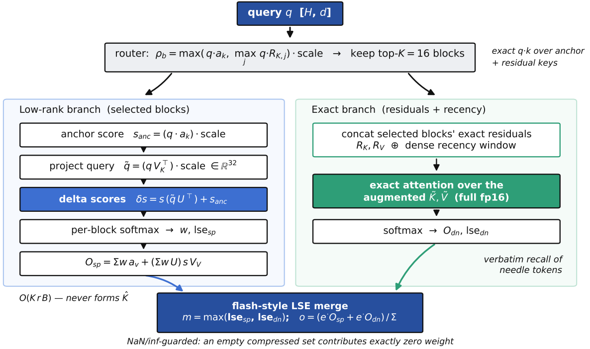
Figure 5 | The routed sparse decode kernel. A cheap exact router keeps the top- K blocks. Their contribution is computed in the rank- r subspace—anchor score plus a projected-query dot with U —without ever forming \hat{K} . In parallel, the selected blocks’ exact residuals and the dense recency window are attended directly. The two halves are combined by a flash-style log-sum-exp merge, guarded so an empty compressed set contributes exactly zero weight.
