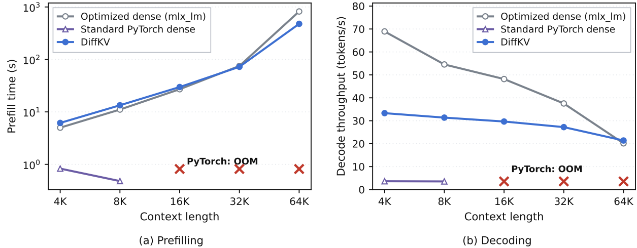
Figure 8 | Prefill and decode of DiffKV against an optimized mlx_lm dense baseline and a standard PyTorch dense baseline on identical int4 weights (Apple M3, 8.6 GB; greedy, 128 decode tokens). (a) Block-sparse prefill grows sub-quadratically, overtakes the optimized dense baseline by 32K, and prefills 1.72× faster at 64K; the standard PyTorch dense is fast at short context but runs out of memory at 16K+ (×). (b) DiffKV decode is nearly flat in context but slower than the optimized dense wherever that cache still fits; the standard PyTorch dense decodes at only ≈3.6 tok/s and OOMs at 16K+.
