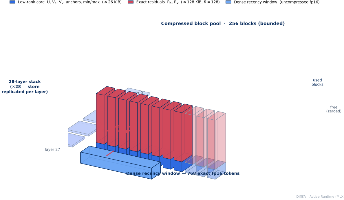
Figure 3. The per-session KV store in three dimensions. The store is replicated across all 28 layers (left). Within a layer, the compressed pool is a bounded array of M=256 block slots; each occupied slot holds a small low-rank core and—at the default budget—a much larger block of exact residuals (residuals dominate the per-block bytes, cf. Table 1). The dense recency window (front) holds the newest 768 tokens uncompressed; when it overflows, its oldest block is flushed and compressed into a pool slot.
