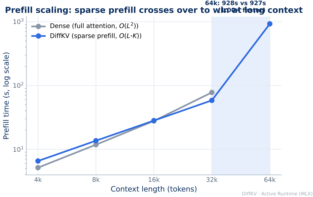
Figure 7. Prefill time vs. context (log scale). Block-sparse prefill grows sub-quadratically and overtakes the dense quadratic baseline at long context; the shaded band marks the region where DIFFKV prefill is faster.
