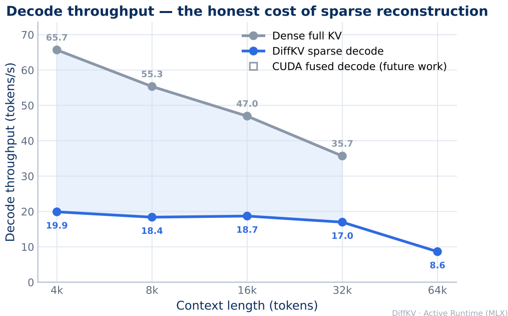
Figure 8. Decode throughput vs. context. Dense is faster wherever its cache fits; DIFFKV’s cached sparse decode is flatter but slower. The CUDA/Triton decode path is reserved for future measurement (§10).
