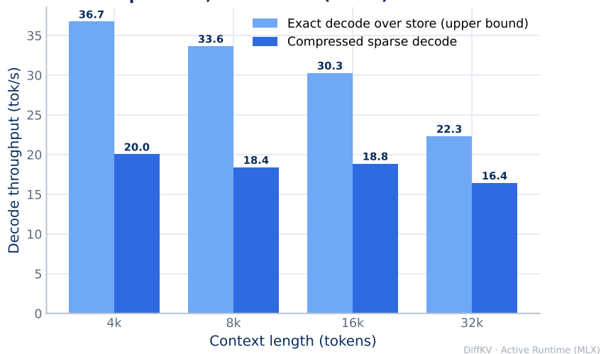
Decode cost of compression, same store ( R = 64 ) — both recover the needle
