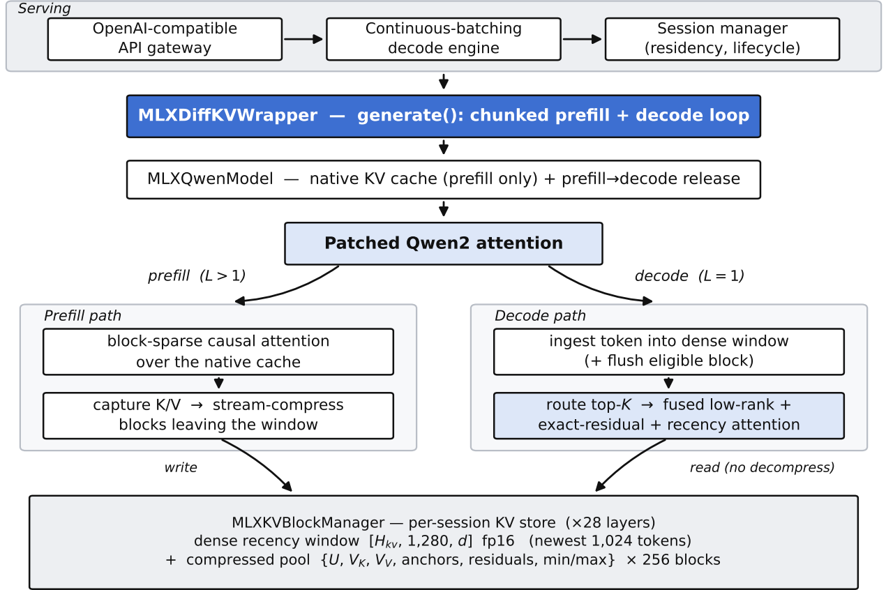
Figure 2 | DKV active-runtime architecture. A serving stack (gateway, batching engine, session manager) drives MLXDiffKVWrapper , which runs chunked prefill and a greedy or sampled decode loop over MLXQwenModel . The model’s attention layer is monkey-patched: on prefill ( L > 1 ) it runs (block-sparse) causal attention over the native cache and captures K/V into the store; on decode ( L = 1 ) it ingests the current token and runs the fused routed sparse attention. All state lives in the per-session MLXKVBlockManager : a dense recency window plus a bounded compressed block pool.
