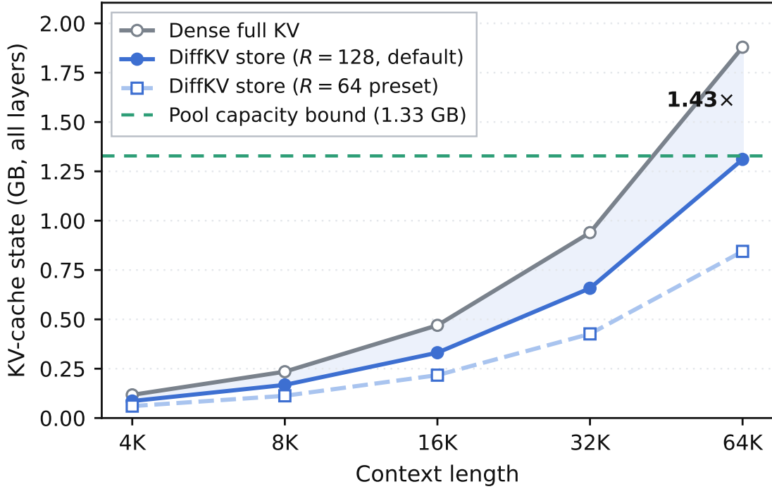
Figure 11 | Analytic KV-state footprint vs. context (whole model). The dense cache grows linearly; the DKV store grows sub-linearly and is bounded by the pre-allocated 256-block pool. Both residual presets are shown; the R=64 preset stays under the pool cap through 64k.
