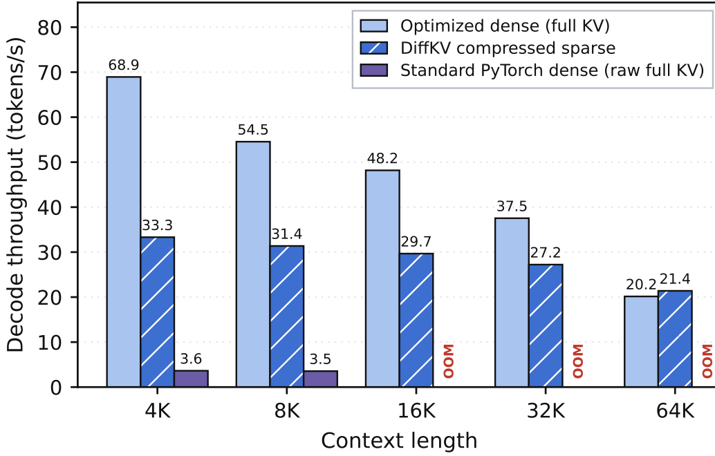
Figure 14 | Decode throughput of the three engines vs. context. DKV’s compressed sparse decode is slower than the optimized dense wherever that cache fits, and the two converge by 64k; the standard PyTorch dense decodes at only \approx 3.6 tok/s and OOMs at 16k+. The same-store compressed-vs-exact mechanism ablation is in Table 4.
