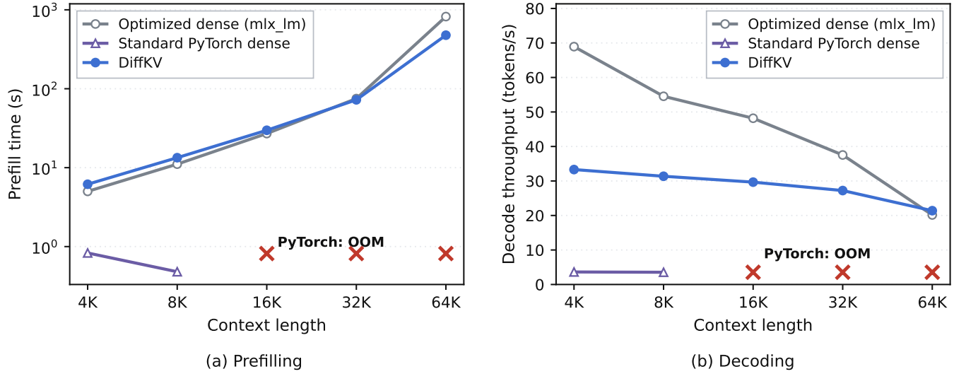
Figure 12 | Prefill and decode of DKV against an optimized mlx_lm dense baseline and a standard PyTorch dense baseline on identical int4 weights (Apple M3, 8.6 GB; greedy, 128 decode tokens). (a) Block-sparse prefill grows sub-quadratically, overtakes the optimized dense baseline by 32K, and prefills 1.72× faster at 64K; the standard PyTorch dense is fast at short context but runs out of memory at 16K+ (×). (b) DKV decode is nearly flat in context but slower than the optimized dense wherever that cache still fits; the standard PyTorch dense decodes at only ≈3.6 tok/s and OOMs at 16K+.
