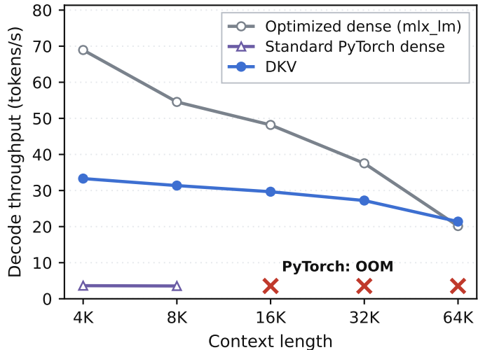
(b) Decoding
