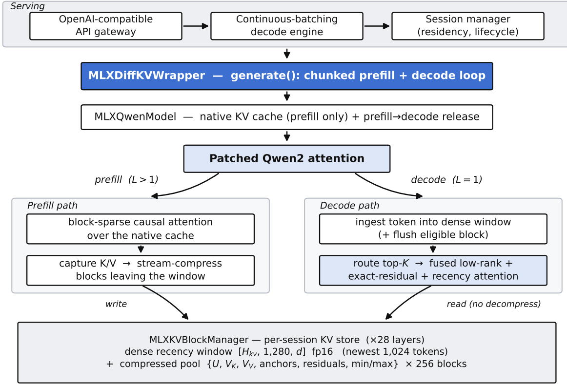
Figure 2 | DKV active-runtime architecture. A serving stack (gateway, batching engine, session manager) drives MLXDiffKVWrapper, which runs chunked prefill and a greedy or sampled decode loop over MLXQwenModel. The model’s attention layer is monkey-patched: on prefill ( L > 1 ) it runs (block-sparse) causal attention over the native cache and captures K/V into the store; on decode ( L = 1 ) it ingests the current token and runs the fused routed sparse attention. All state lives in the per-session MLXKVBlockManager: a dense recency window plus a bounded compressed block pool.
