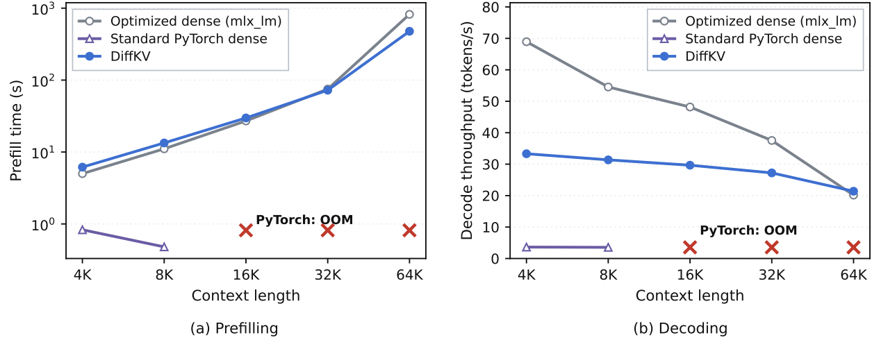
Figure 13 | Prefill and decode of DKV against an optimized mlx_lm dense baseline and a standard PyTorch dense baseline on identical int4 weights (Apple M3, 8.6GB; greedy, 128 decode tokens). (a) Block-sparse prefill grows sub-quadratically, overtakes the optimized dense baseline by 32K, and prefills 1.72 \times faster at 64K; the standard PyTorch dense is fast at short context but runs out of memory at 16K+ ( \times ). (b) DKV decode is nearly flat in context but slower than the optimized dense wherever that cache still fits; the standard PyTorch dense decodes at only \approx 3.6 tok/s and OOMs at 16K+.
