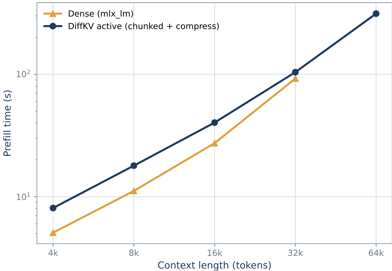
Prefill time vs context
