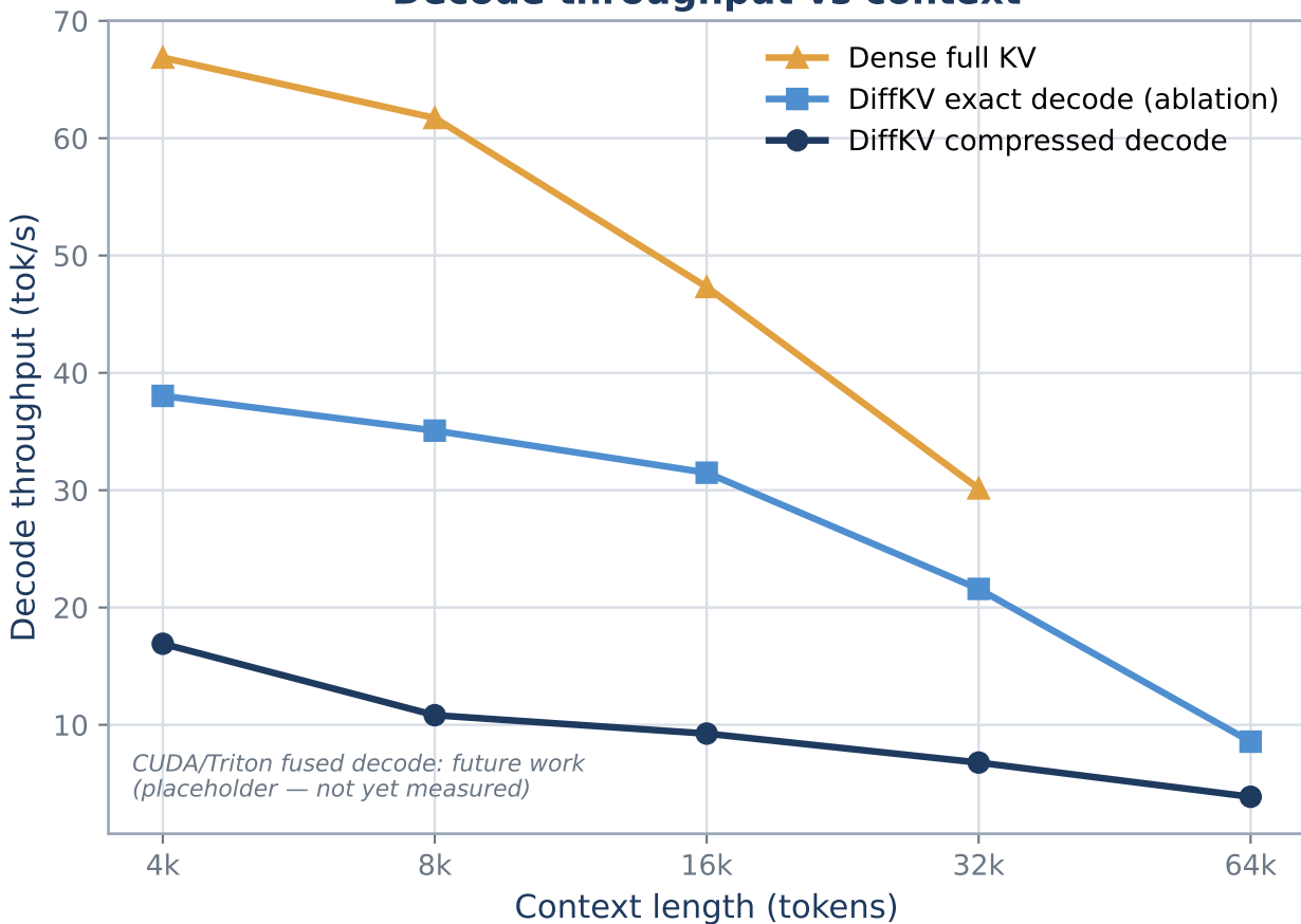
Decode throughput vs context
