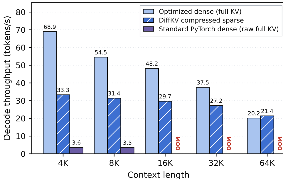
Figure 10 | Decode throughput of the three engines vs. context. DKV’s compressed sparse decode is slower than the optimized dense wherever that cache fits, and the two converge by 64k; the standard PyTorch dense decodes at only \approx 3.6 tok/s and OOMs at 16k+. The same-store compressed-vs-exact mechanism ablation is in Table 4.
