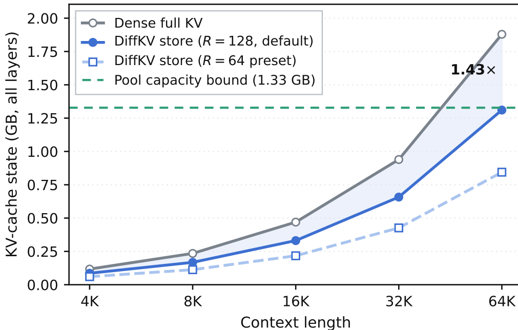
Figure 7 | Analytic KV-state footprint vs. context (whole model). The dense cache grows linearly; the DKV store grows sub-linearly and is bounded by the pre-allocated 256-block pool. Both residual presets are shown; the R=64 preset stays under the pool cap through 64k.
