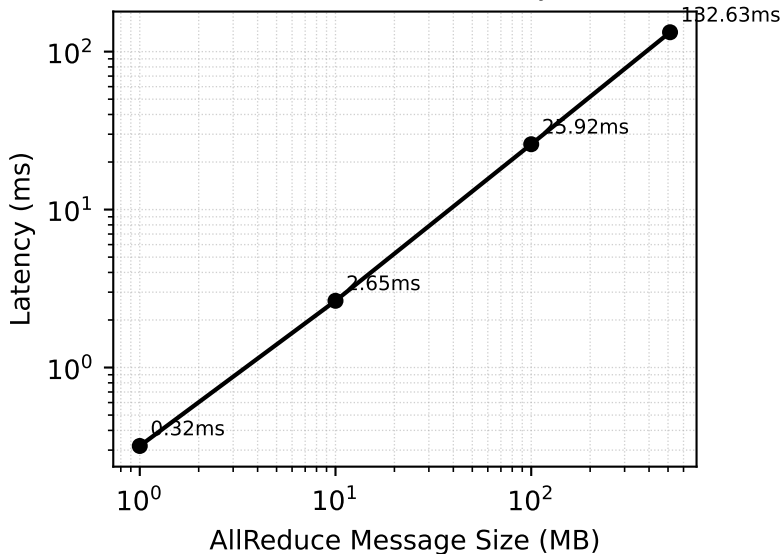
NCCL AllReduce Latency
