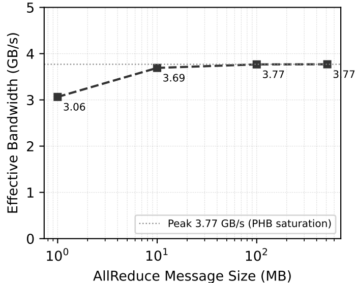
NCCL AllReduce Effective Bandwidth
