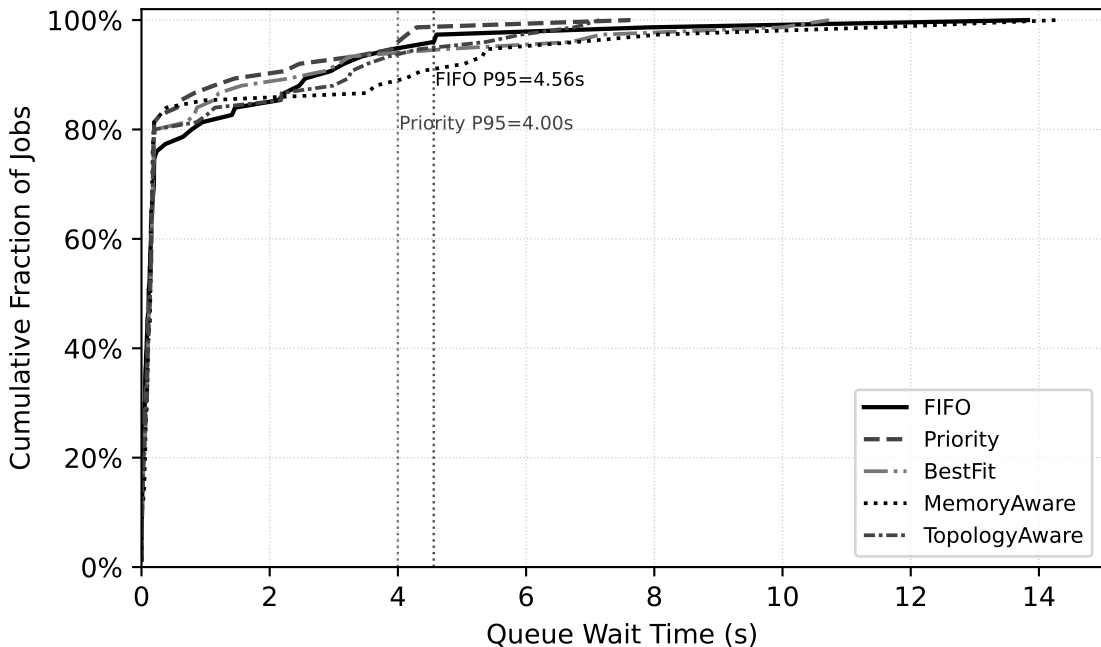
CDF of Per-Job Queue Wait Time by Scheduler (15 jobs \times 5 trials, uniform arrivals, dual T4)
