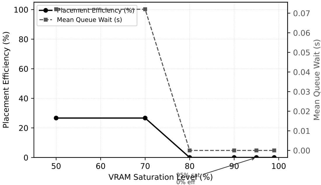
VRAM Saturation vs. Placement Efficiency (MemoryAwareScheduler)
