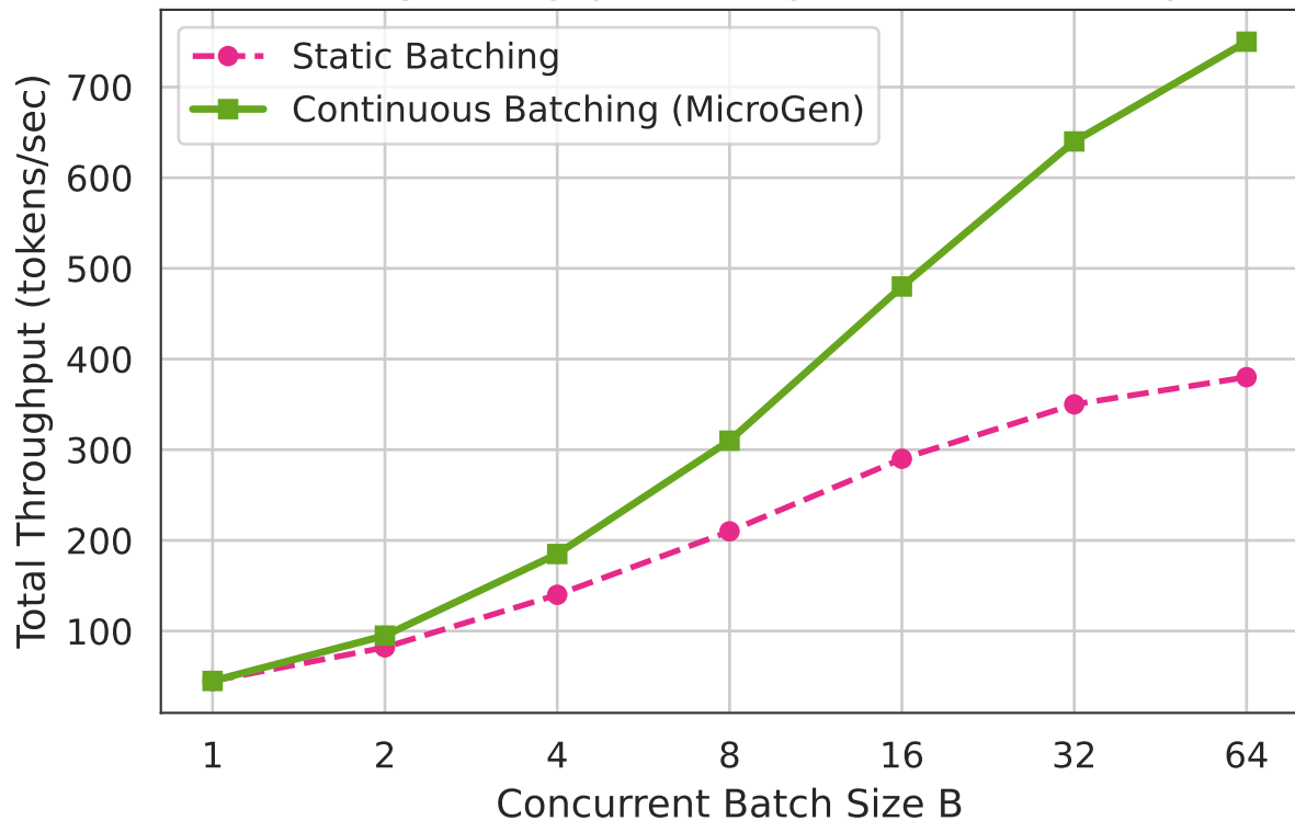
Serving Throughput Scaling under Concurrency
