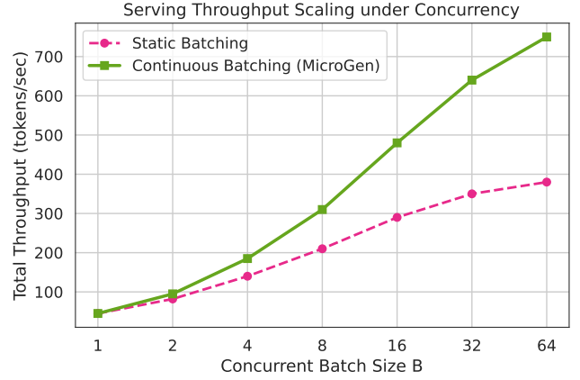
Figure 4: Serving throughput (tokens/sec) and average TPOT latency scaling under increasing request concurrency batch sizes ( B = 1 to B = 64 ).
