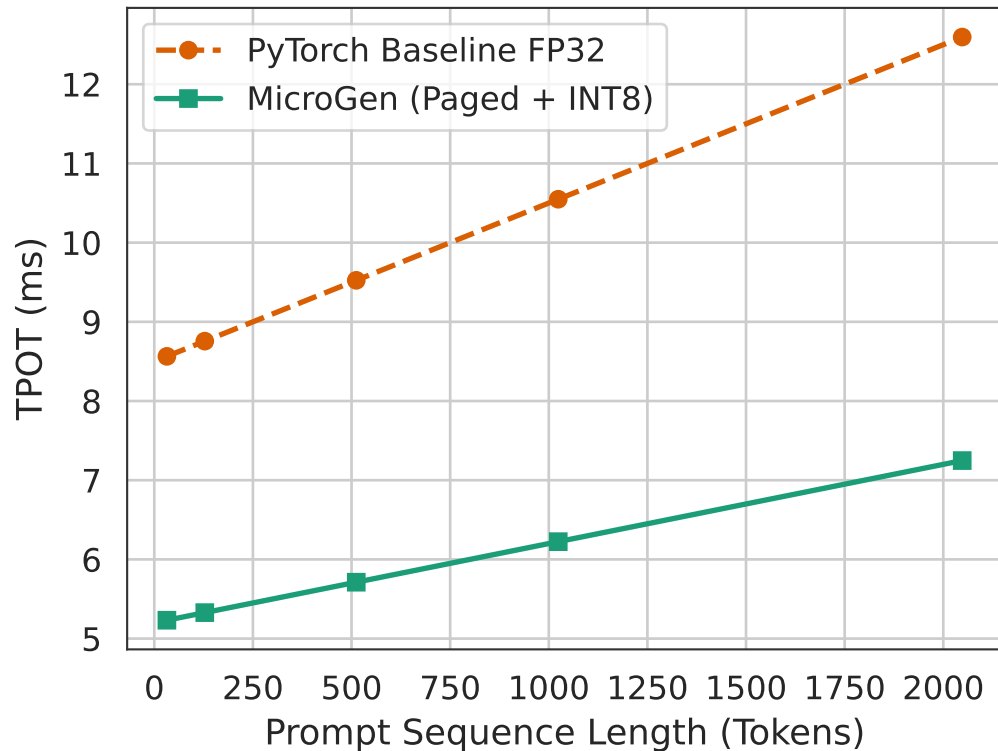
(b) Time Per Output Token (TPOT)
