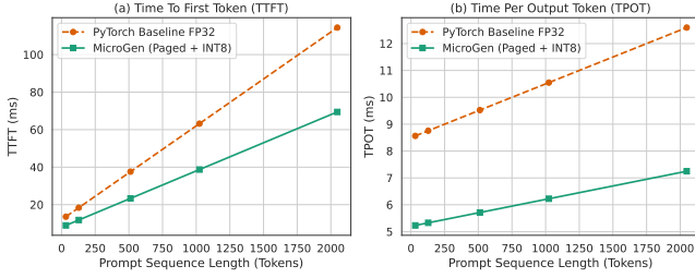
Figure 5: TTFT and TPOT latency scaling across prompt context lengths for sshleifer/tiny-gpt2 and gpt2 (124M) models.
