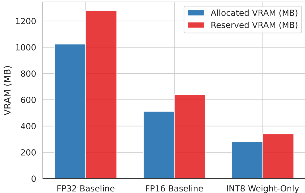
Memory Compression Pareto Breakdown
