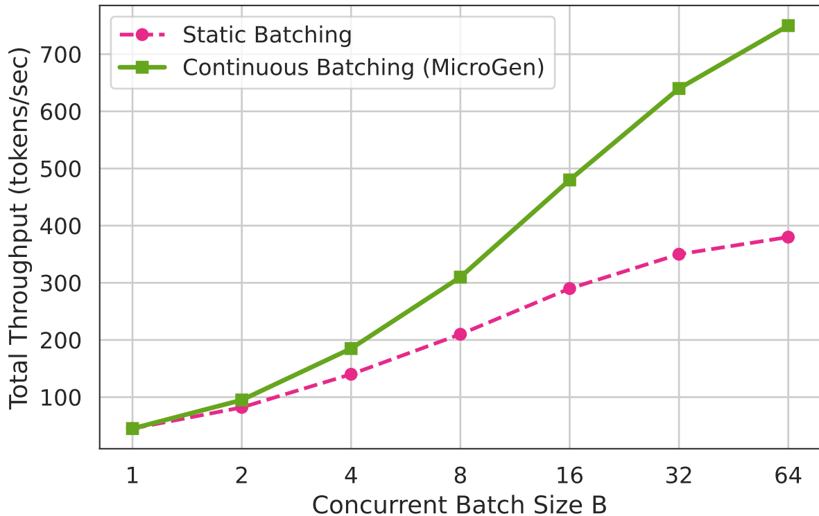
Serving Throughput Scaling under Concurrency
