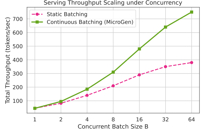
Figure 4: Serving throughput (tokens/sec) and average TPOT latency scaling under increasing request concurrency batch sizes ( B = 1 to B = 64 ).
