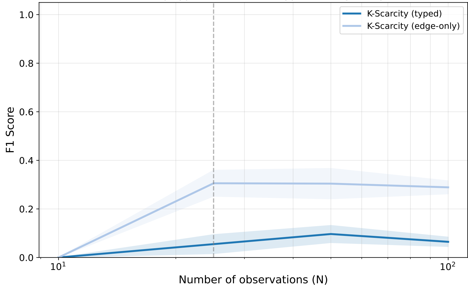
Relationship Type Identification: Typed vs Edge-Only F1
