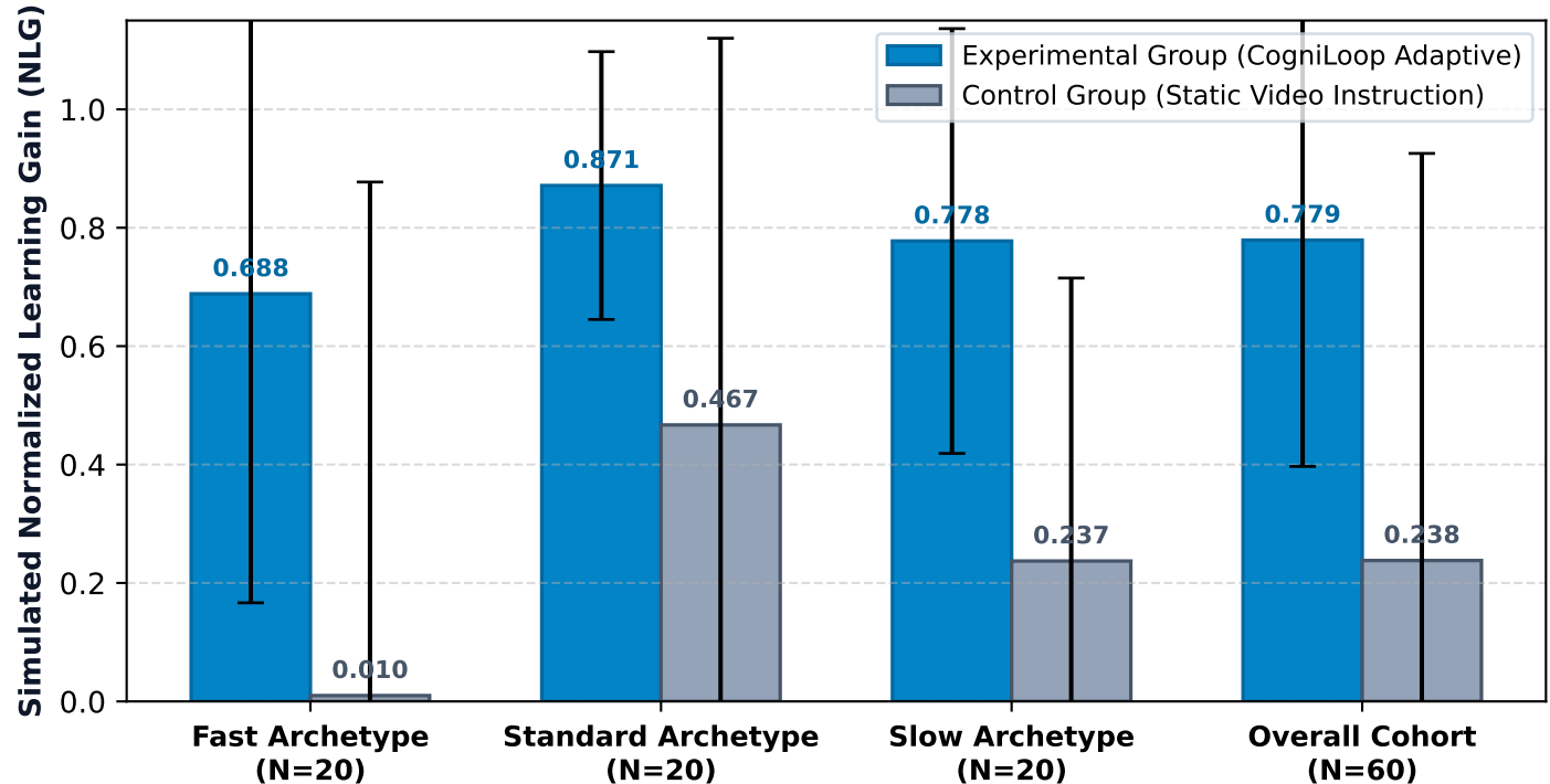
Simulated Normalized Learning Gain Across Archetypes (Welch's t = 3.768 , p < 0.001 , d = 0.973 )
