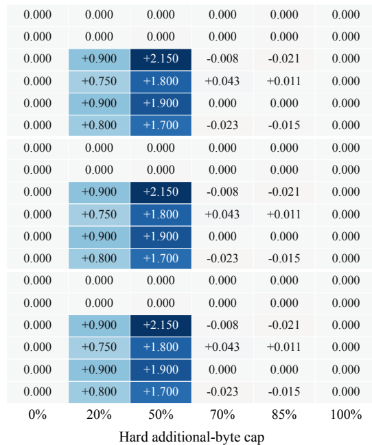
(b) Minimax minus balanced
