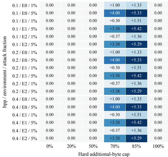
(a) Minimax minus best fixed
