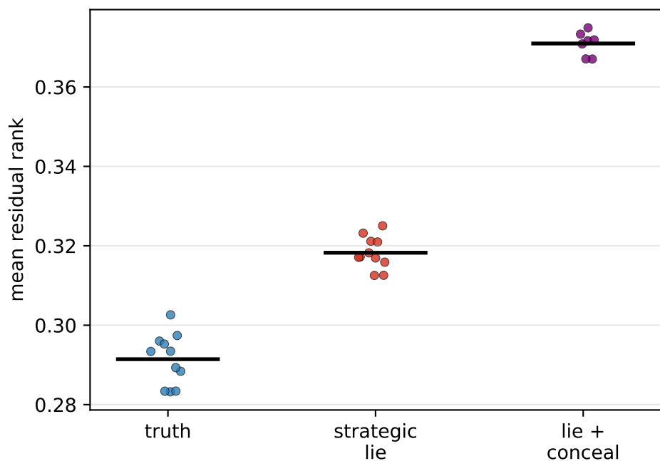
Phi-3-mini: self-constructed lie detected (AUC 1.0); concealment does not reduce it
