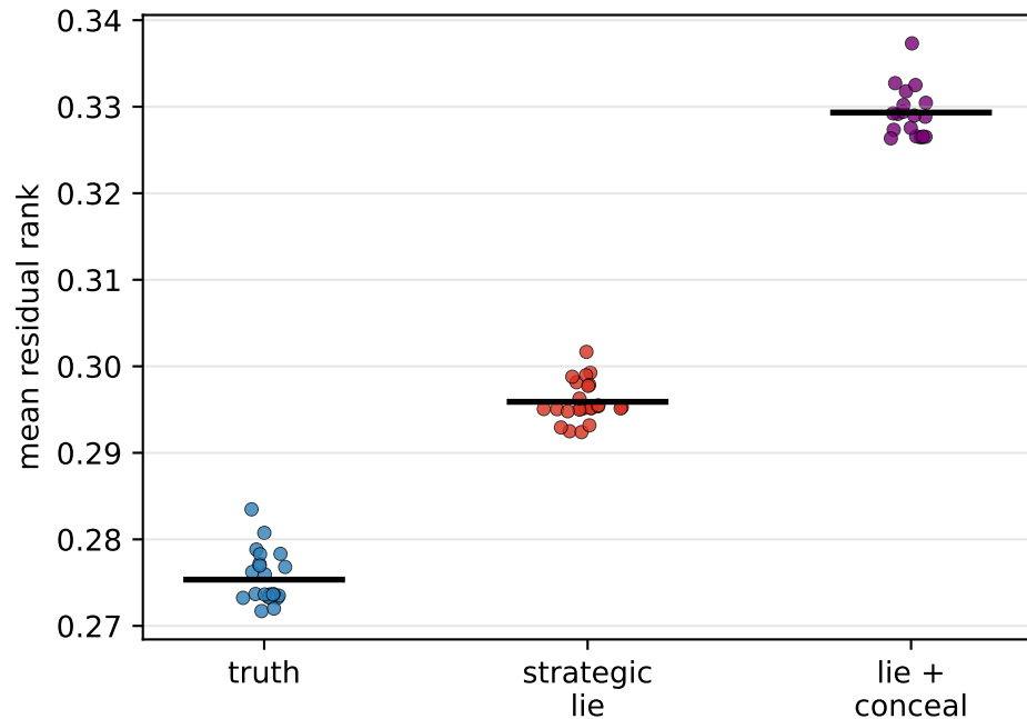
Qwen2.5-7B: self-constructed lie detected (AUC 1.0); concealment does not reduce it
