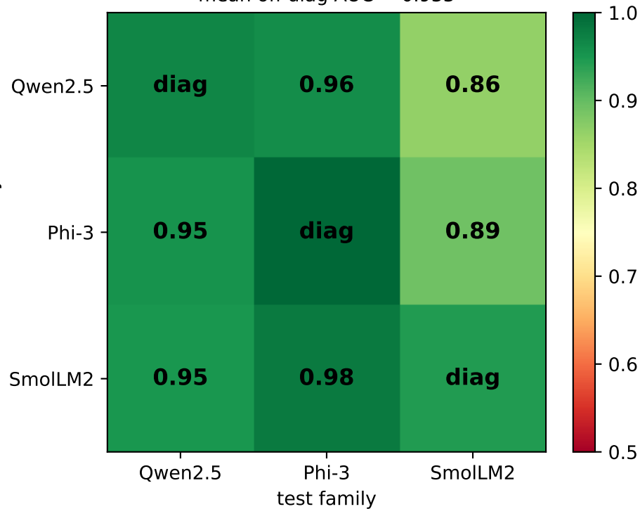
Cross-family transfer (same format) mean off-diag AUC = 0.933
