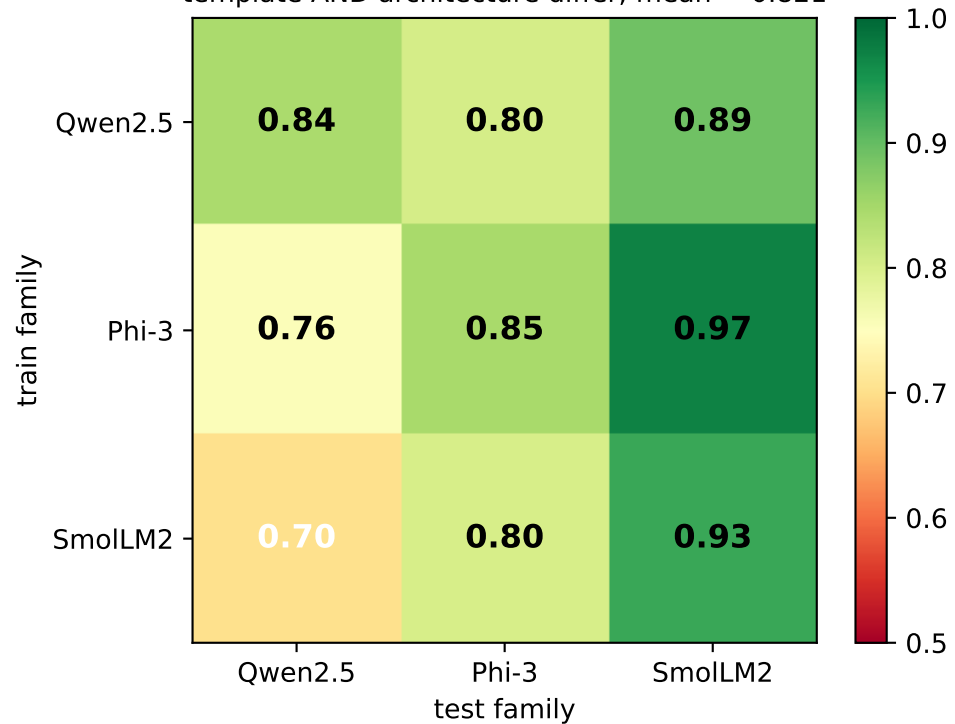
Cross-format + cross-family template AND architecture differ; mean = 0.821
