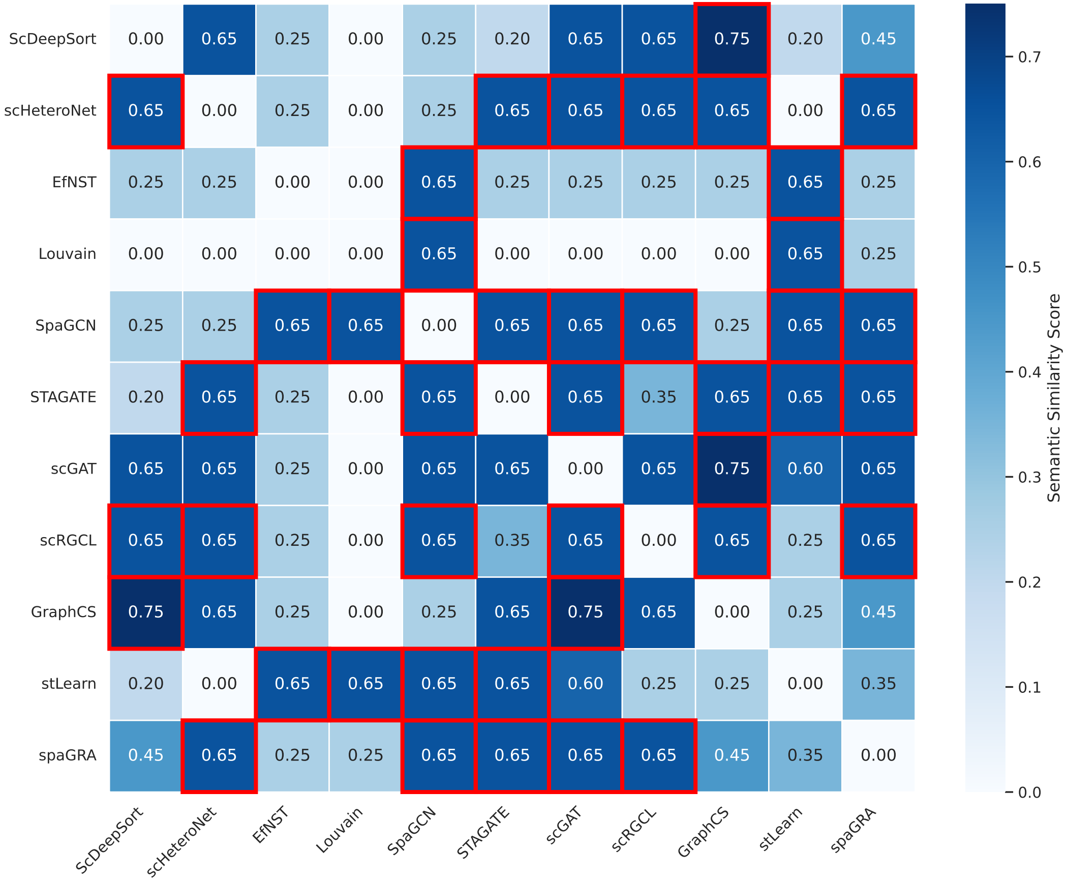
Model-to-Model Similarity Landscape & Retrieval Trajectory
