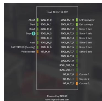
Factory I/O Drivers
