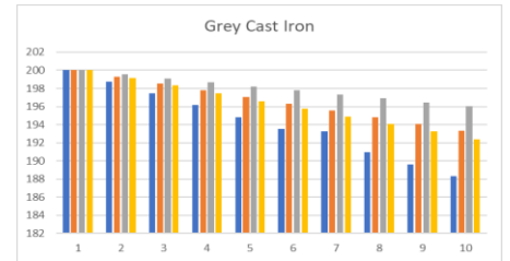
Temp fall graph – Grey Cast Iron
