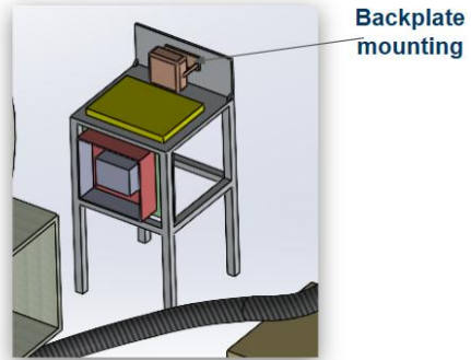
Layout 2 - HMI Screen on a backplate
