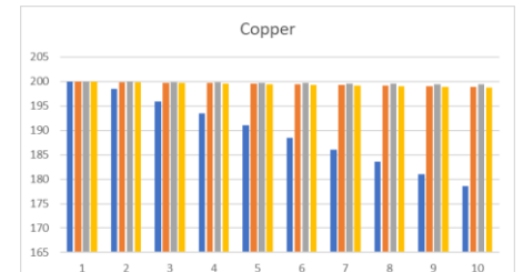
Temperature fall graph – Copper
