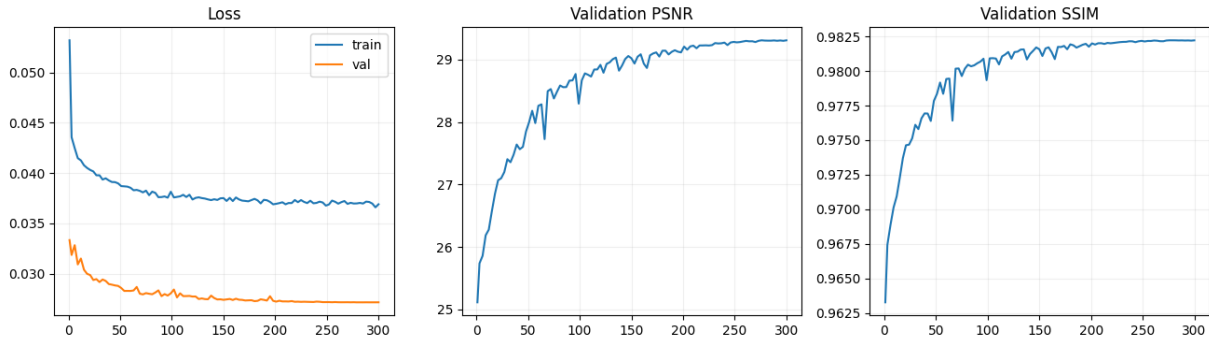
Figure 2. EDSR training loss and validation fidelity across 300 epochs.
