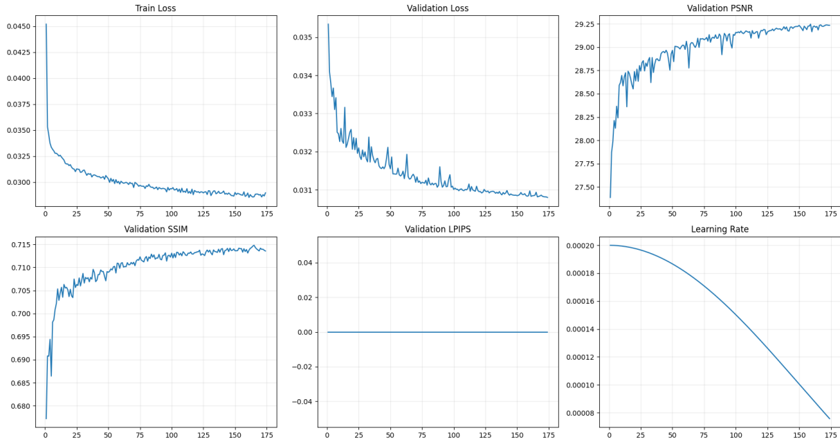
Figure 4. RCAN convergence and cosine learning-rate schedule; validation LPIPS was recorded as a zero placeholder during training.
