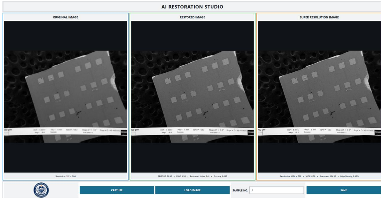
Figure 9. Final native desktop interface showing the three-stage SEM restoration workflow.
