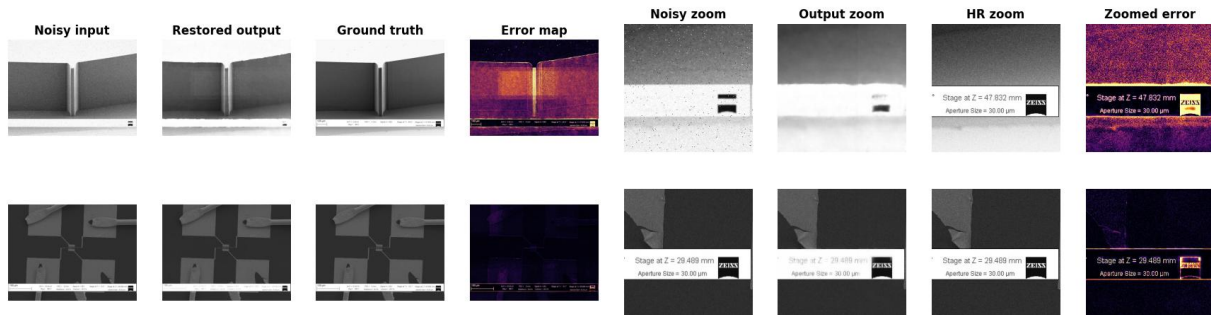
Figure 8. Representative NAFNet notebook test comparisons and error maps (cropped from executed output).
