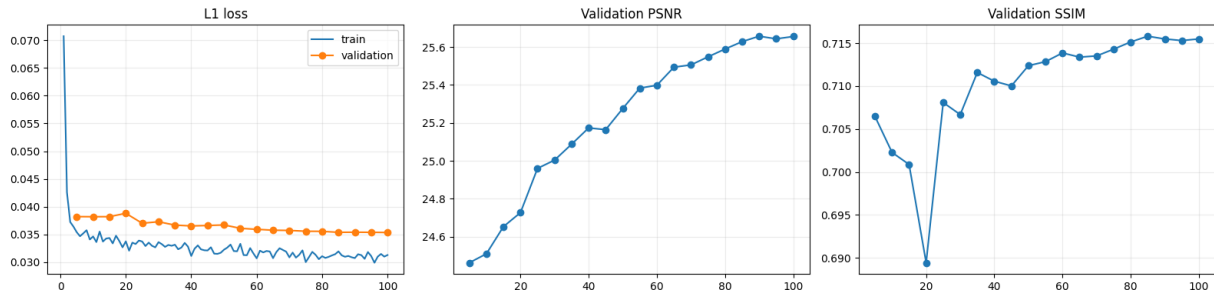
Figure 6. Lightweight SwinIR learning curves with periodic subset validation.
