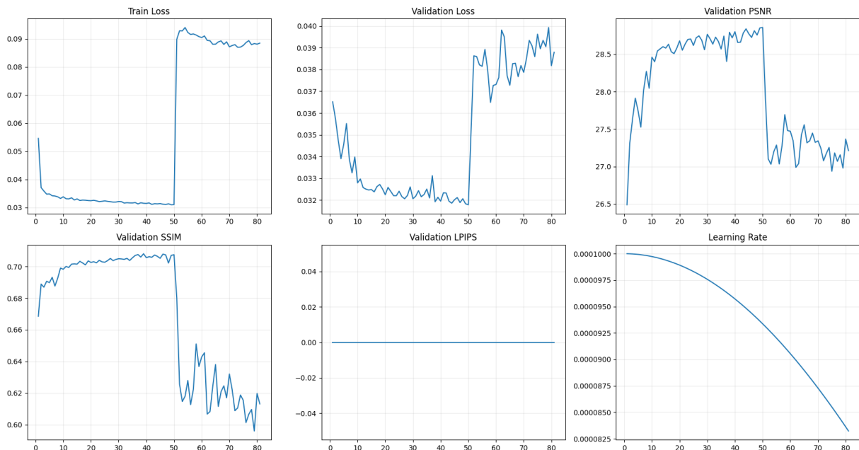
Figure 5. ESRGAN stage transition at epoch 51 and the corresponding fidelity decline.
