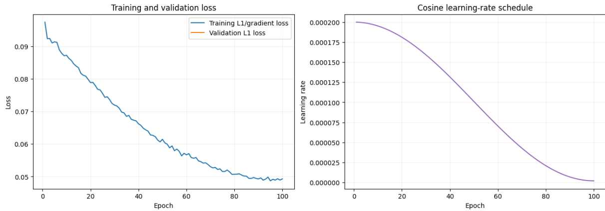
Figure 7. NAFNet training loss and cosine learning-rate schedule.
