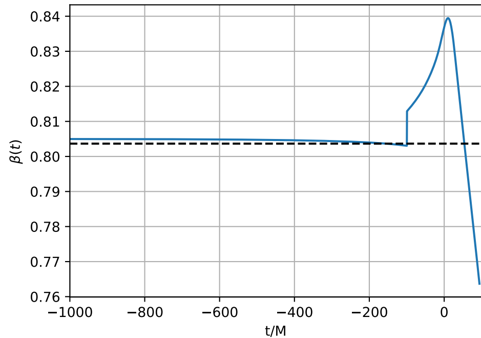
PN-loss Agentic fit ( q = 5 )
