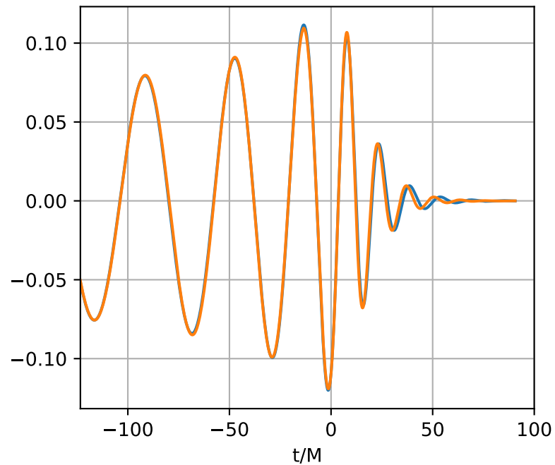
PN-opt q-dependent Agentic fit ( q = 10 ); \text{mathcal{E}} = 0.000272
