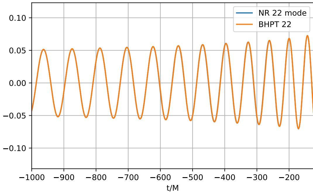
PN-opt q-dependent Agentic fit ( q = 10 ); \text{mathcal{E}} = 0.000272
