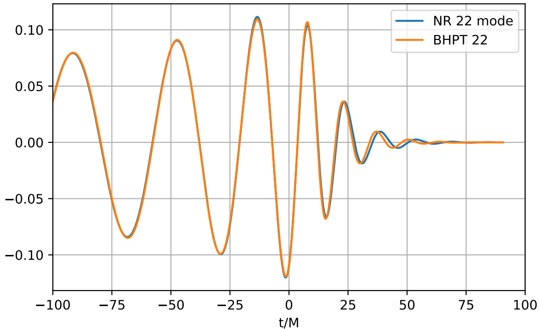
PN-opt q-dependent Agentic fit ( q = 10 )
